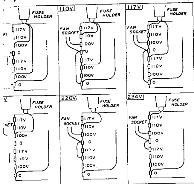
POWER TRANSFORMER CONNECTIONS
